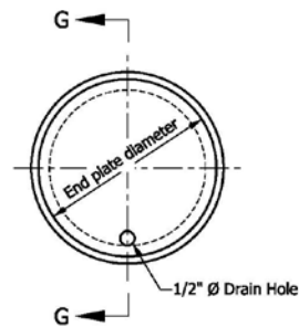
CHORD END PLATE DETAIL
