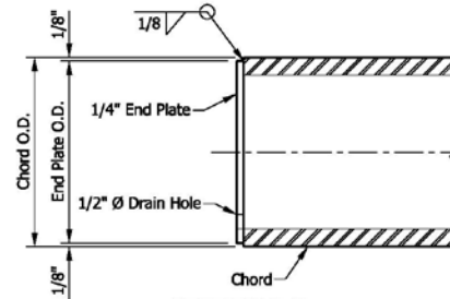
SECTION G-G
