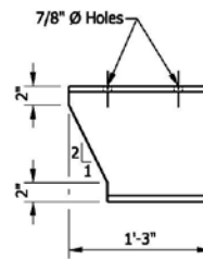
W-BEAM DETAIL
