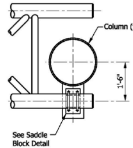
VIEW C-C
