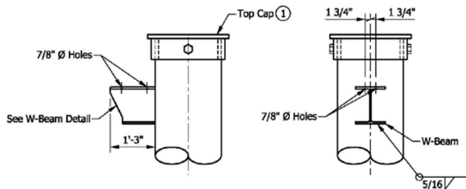
TRUSS SEAT DETAIL
